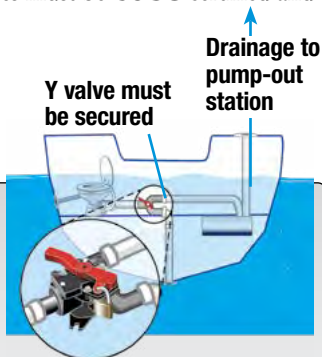
Typical Marine Sanitation Device
